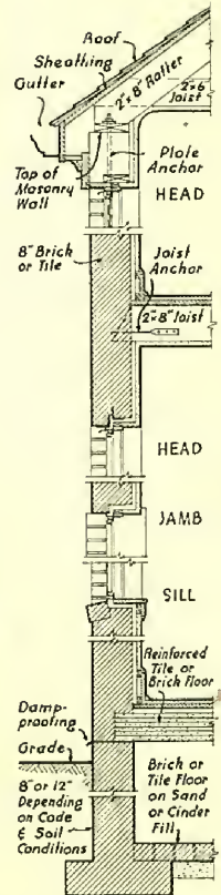
Wall Section
